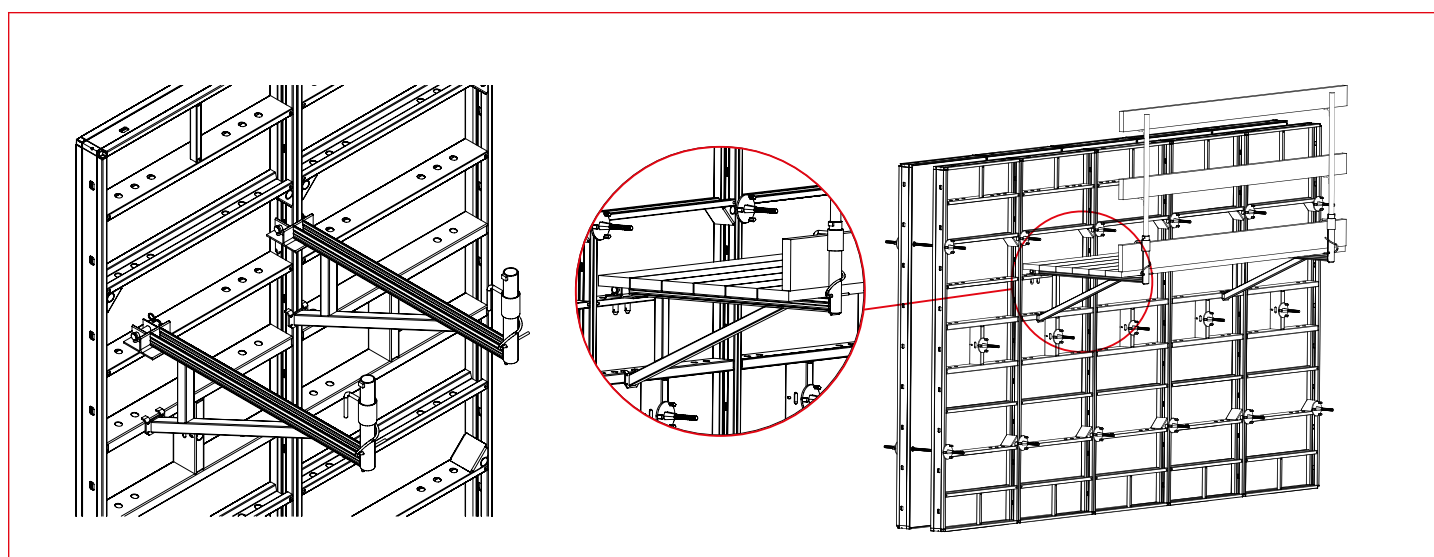
Diagram – working platform assembly
