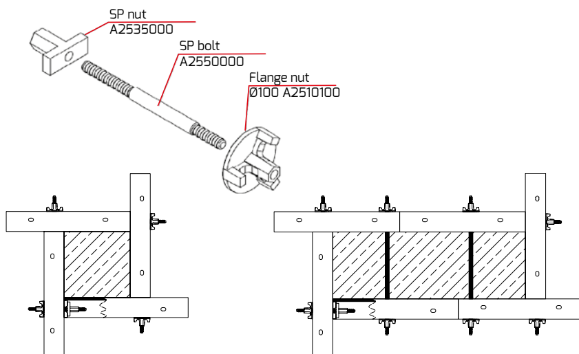
Board connecting diagram
