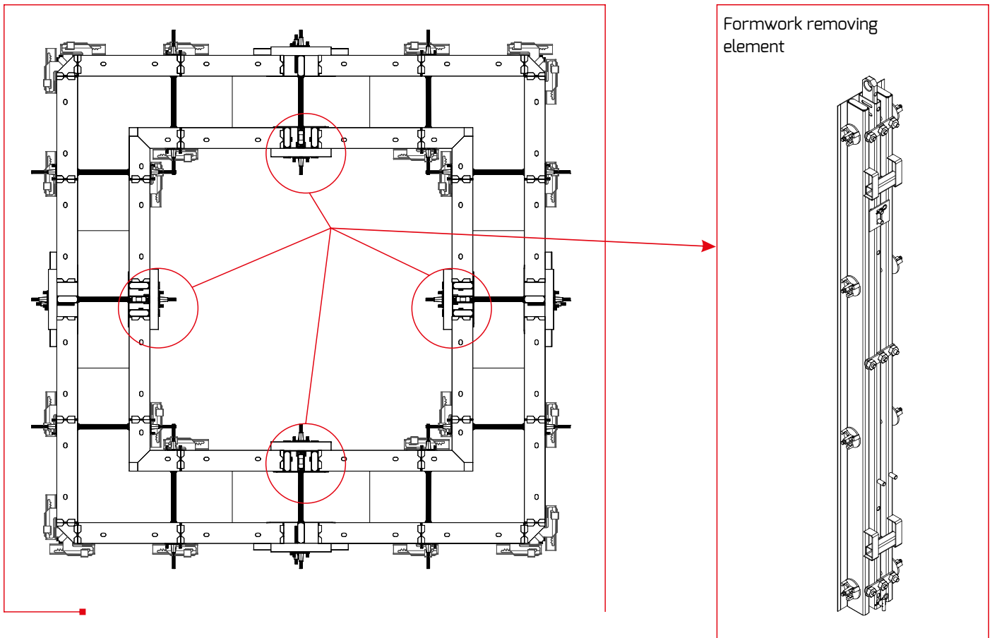
Lift shaft's Formwork
